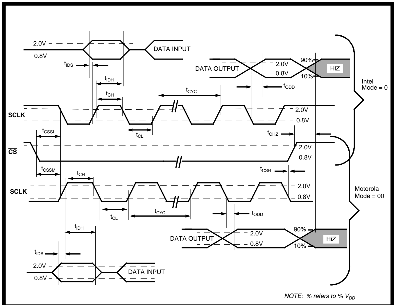
Figure 14 - Microport Timing
