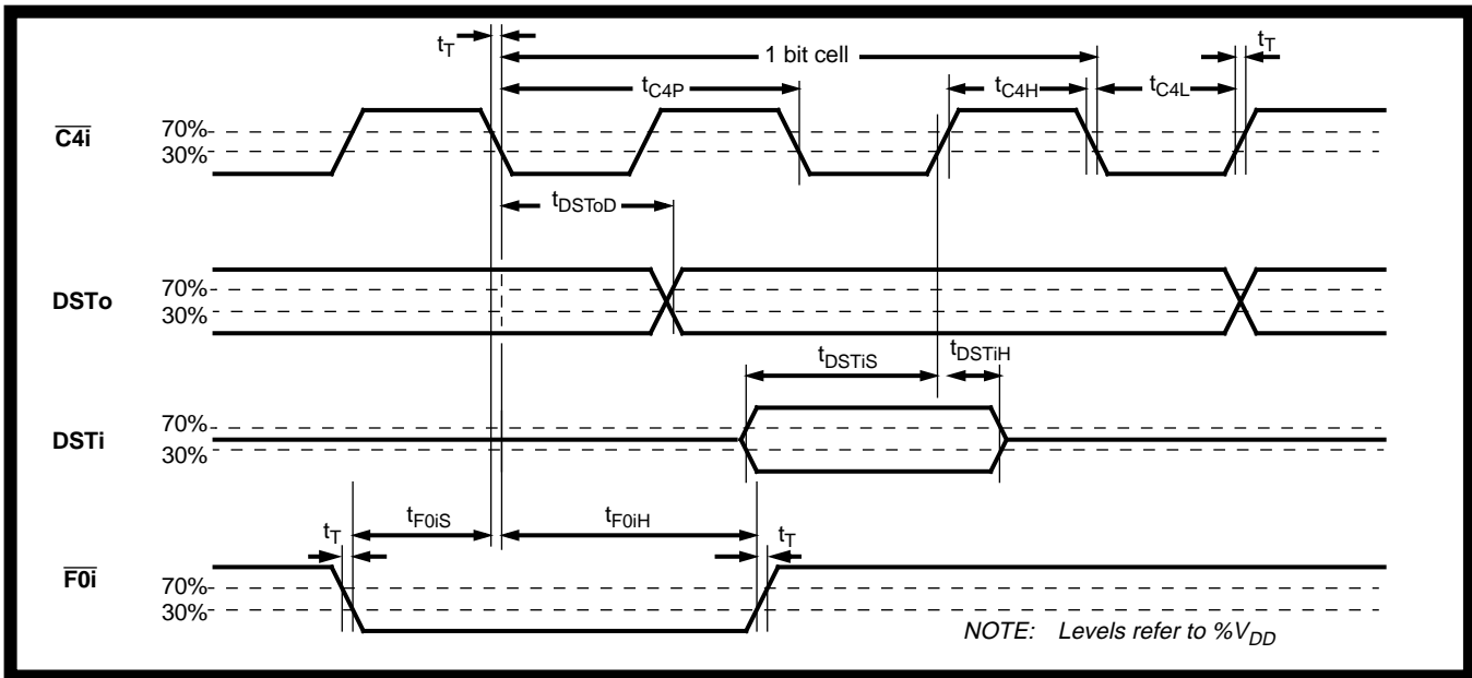
Figure 11 - ST-BUS Timing Diagram
