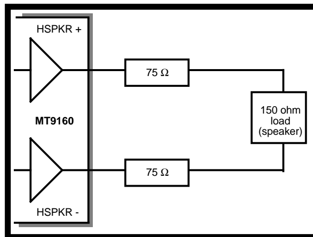
Figure 4 - Handset Speaker Driver
